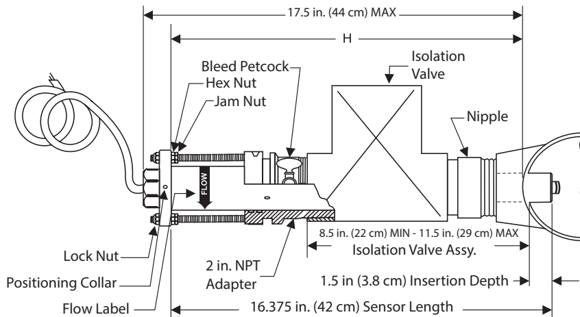
Figure 1: 225/226 Dimensions
