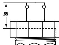
(4) PIN BEND STYLE ELECTRICAL TERMINATION SHELL SIZE 8 (B4), (H1), (L1), (P2)
