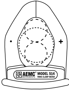
Models 511, 512 & 514 Jaw Opening: 1.575" (40mm) Conductor Size: one 750kcmil cable or two 350kcmil cables
