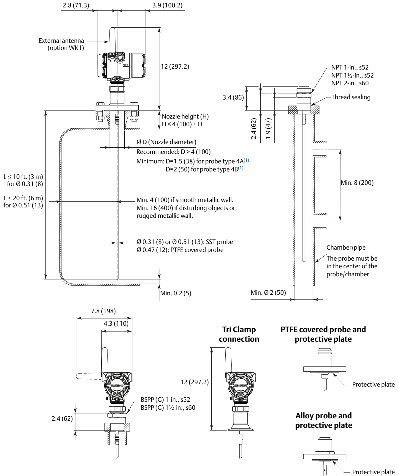
Figure 16. Rigid Single Lead Probe
