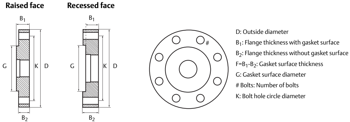
Figure 22. Proprietary Flanges
