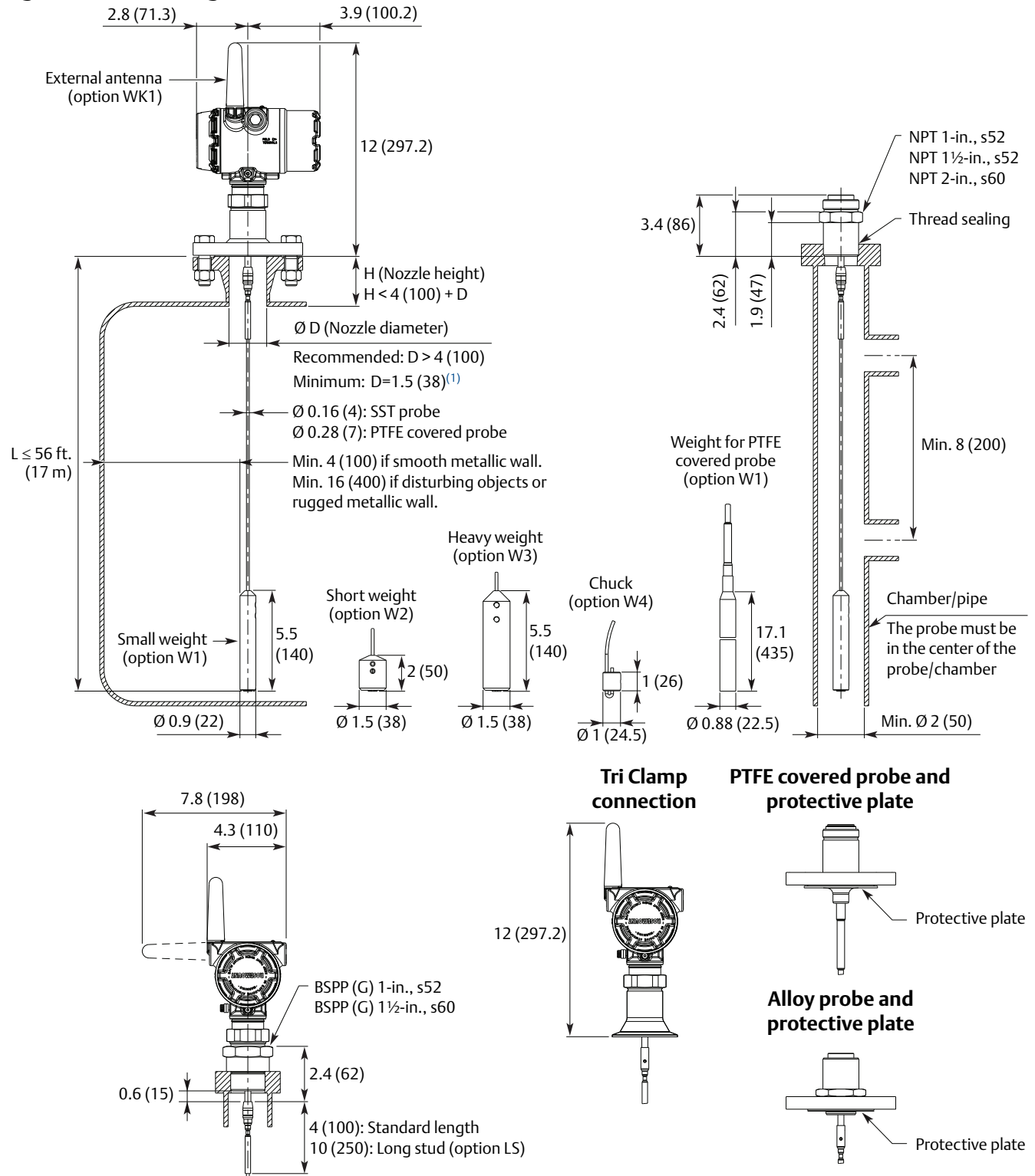
Figure 15. Flexible Single Lead Probe
