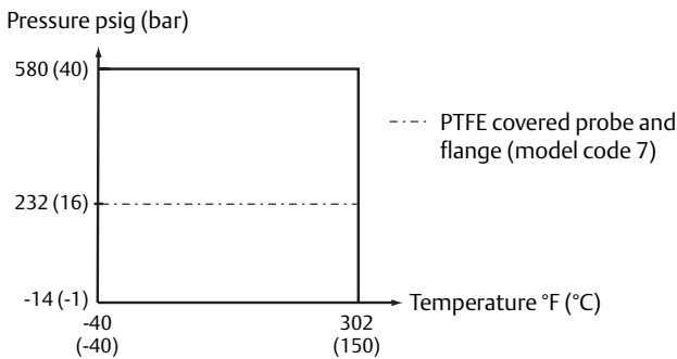
Figure 7. Max. Rating, Standard Tank Connections
