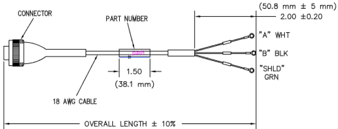
Figure 11: Short Run Interconnect Cable
