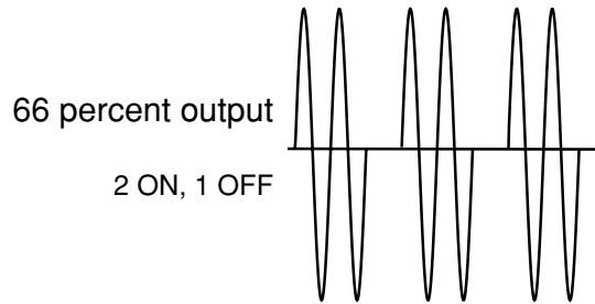
Figure 5.8a Burst fire.
