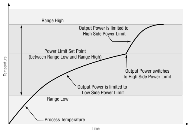
Figure 5.2b Power limits.
