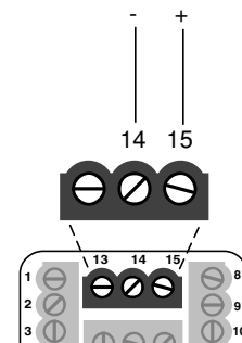
Figure 3.4d – 0-5V=, 1-5V= and 0-10V= (dc) Process
