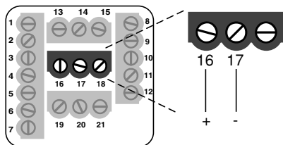
Figure 3.5d – 0-5V \overline{=} , 1-5V \overline{=} and 0-10V \overline{=} (dc) Process
