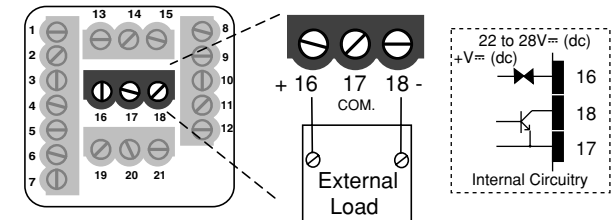
Figure 3.5b – Switched DC, Open Collector
