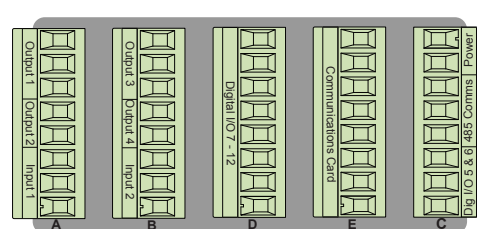
Back View Slot Orientation 1/8 DIN Horizontal PM9
