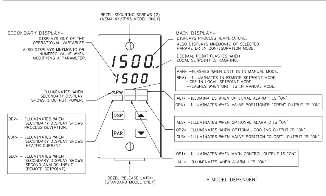
Figure 11, Front Panel
