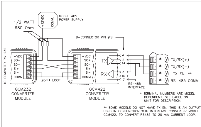
Figure 24, Computer Interface
