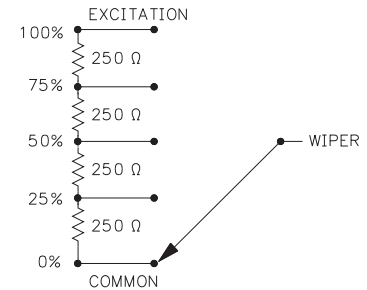
Figure 45, Resistor Divider
