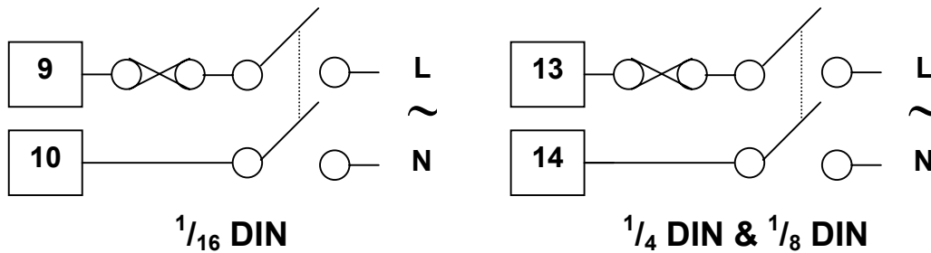
Figure 13. Mains Power Connections
