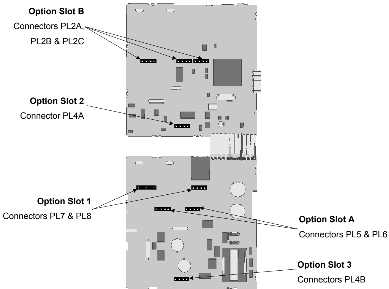
Figure 8. Option Module Connectors - 1/8 & 1/4 DIN Instruments
