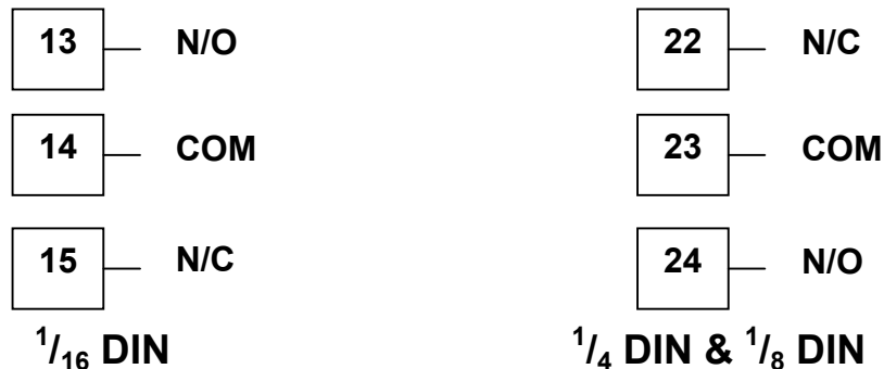
Figure 22. Option Slot 2 - Relay Module
