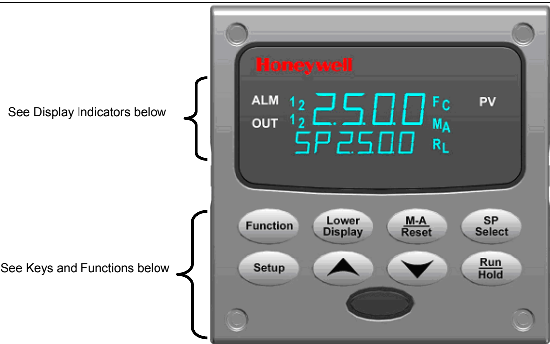
Figure 2—Operator Interface (all display indicators shown)
