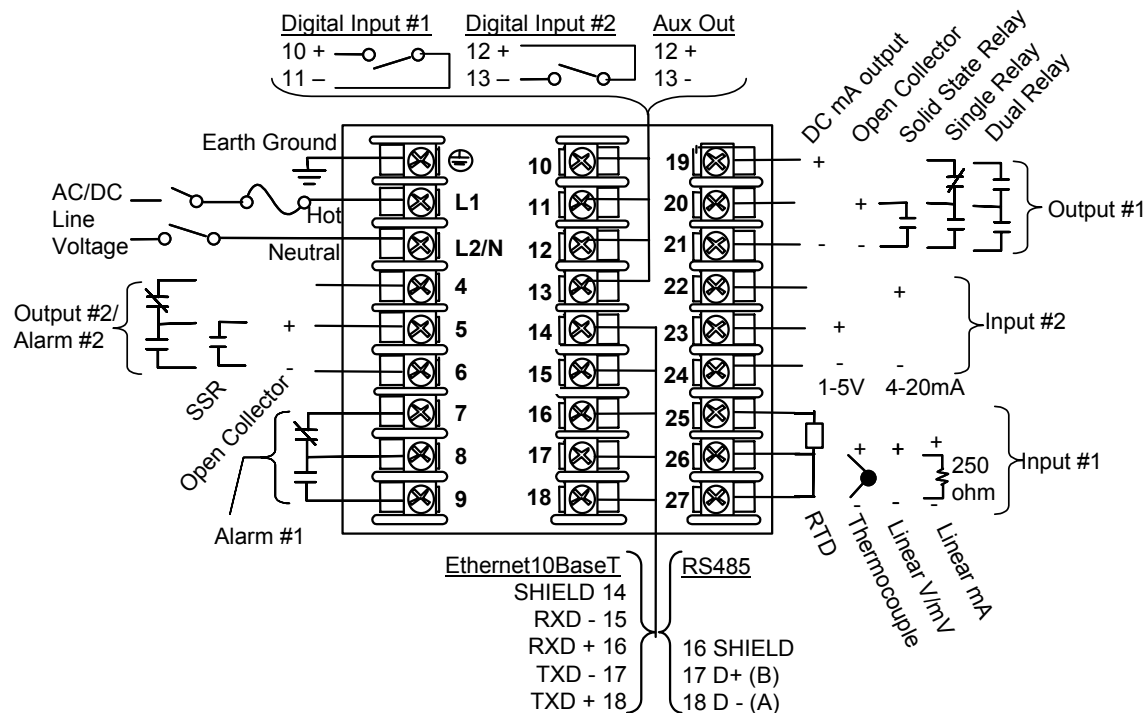
Figure 6—External Wiring Diagram
