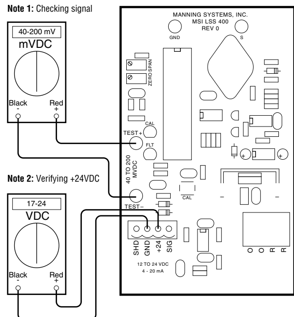
Figure 6: Troubleshooting the 4/20 mA Vent Line Sensor and Pre-Amp
